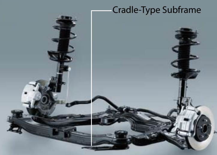
MacPherson-Strut Front Suspension
